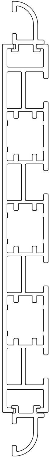
Light Box Double Side finishing on the side Ts Master 160 + Ts 90 +Ts 90
