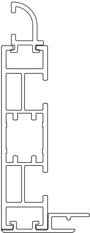
LED Light Box Finishing on the Side Ts Master 80 + Ts Back + Ts 90
