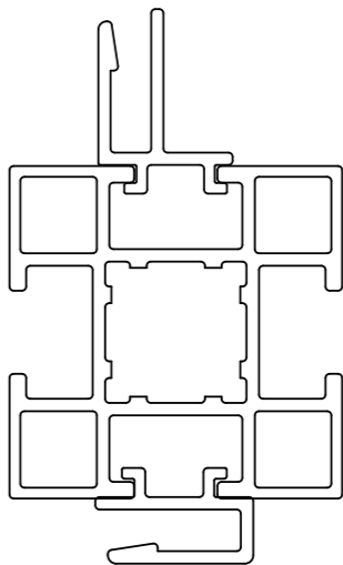
Support Textile Application Ts Mod 40x40 + Ts 90T + Ts FT
