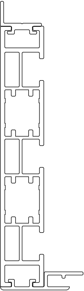
Panel Light Box Finish on the Side Ts Master 120 + Ts Back +Ts C10
