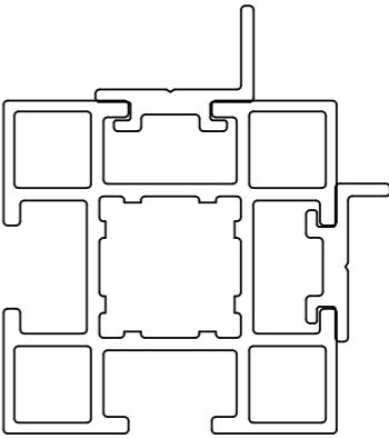
Support Panel Application Ts Mod 40x40 + Ts C5 + Ts C10
